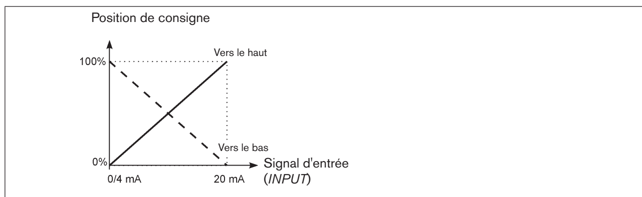
Figure 49 : Diagramme DIR.CMD
