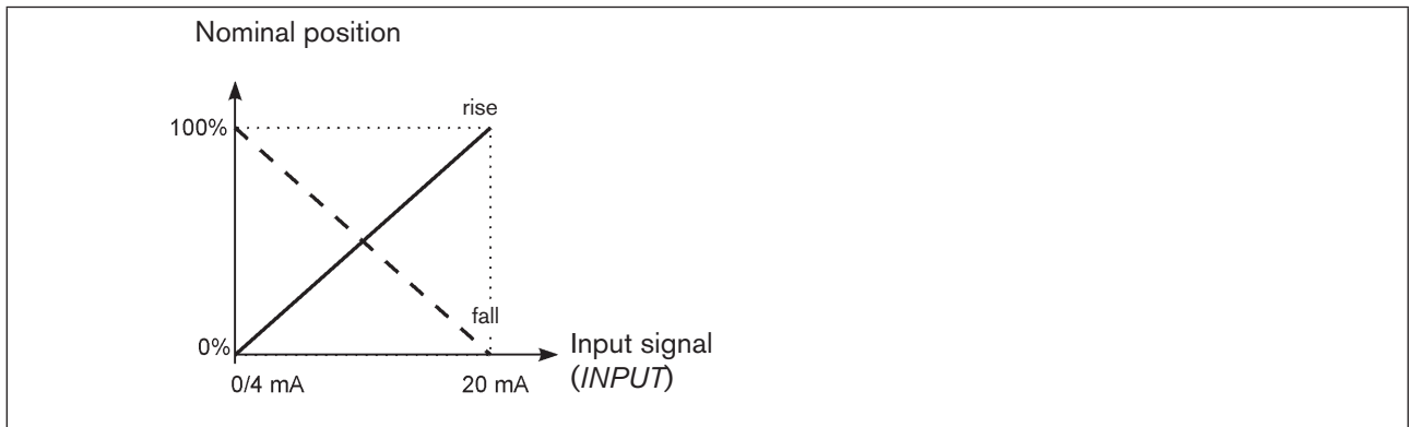
Figure 49: DIR.CMD graph
