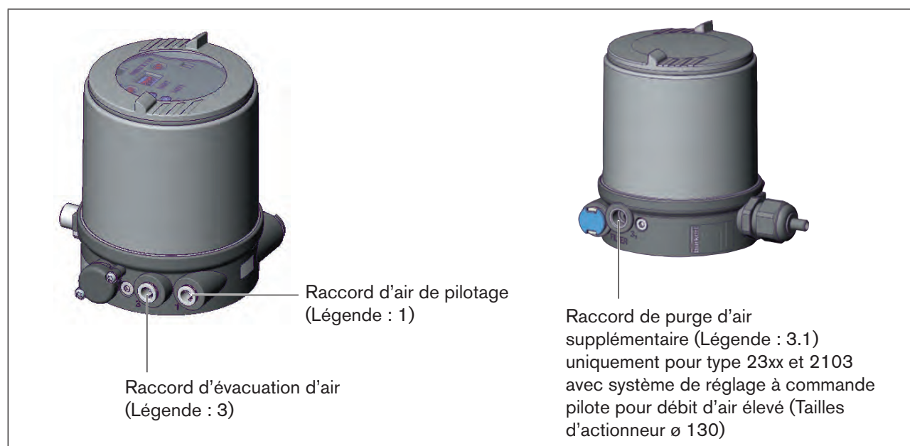
Figure 32 : Raccordement pneumatique
