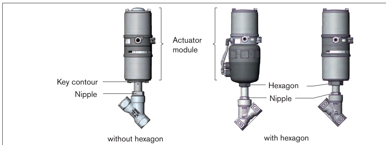
Figure 29: Rotating the actuator module
