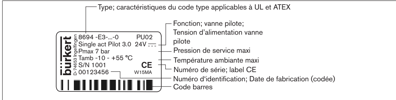
Figure 8 : Plaque signalétique UL
