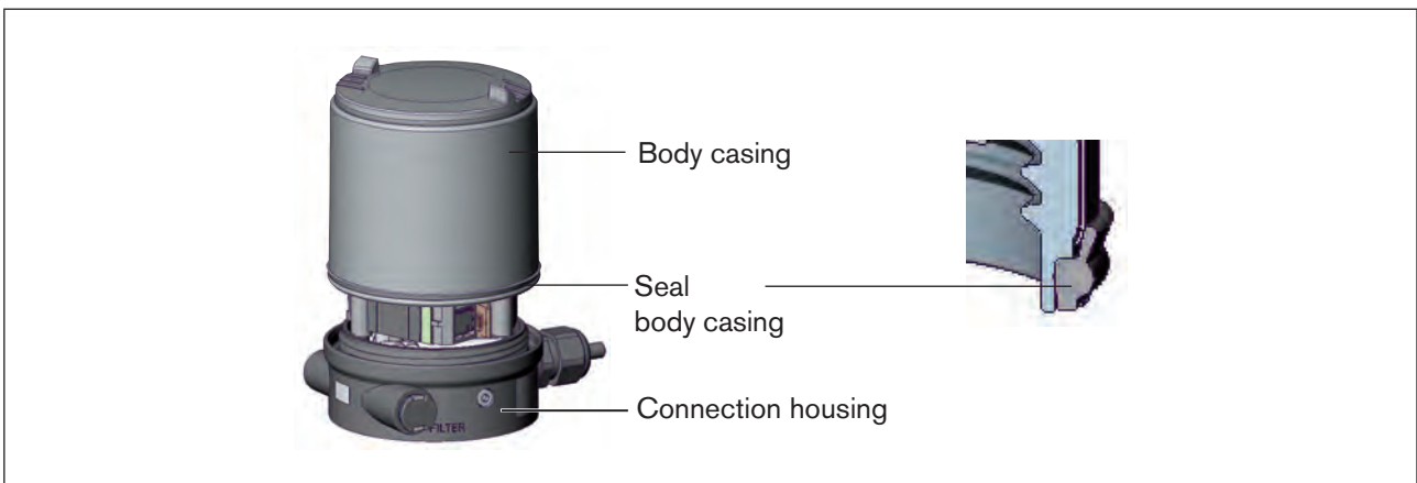
Figure 17: Position of the seal in the body casing
