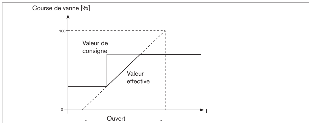
Figure 56 : Diagramme X.TIME
